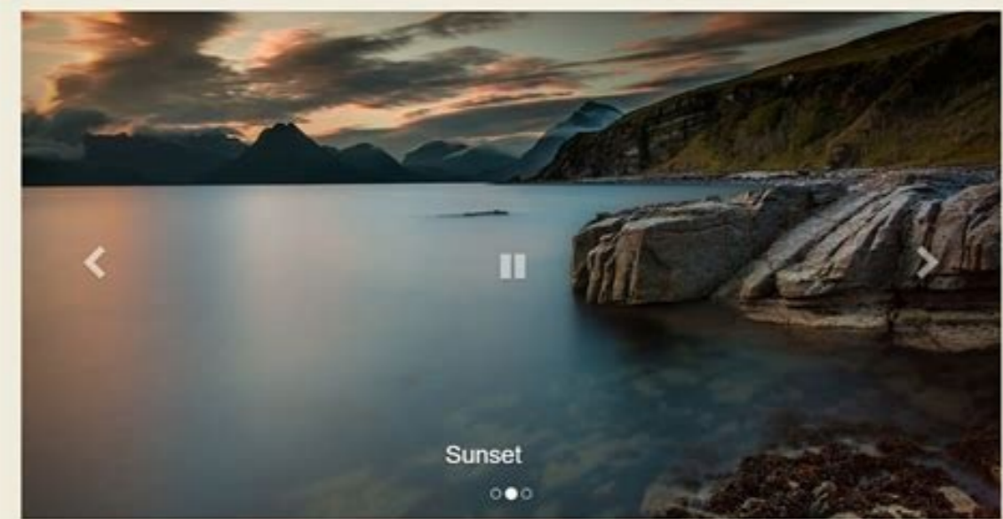
Bootstrap Carousel
